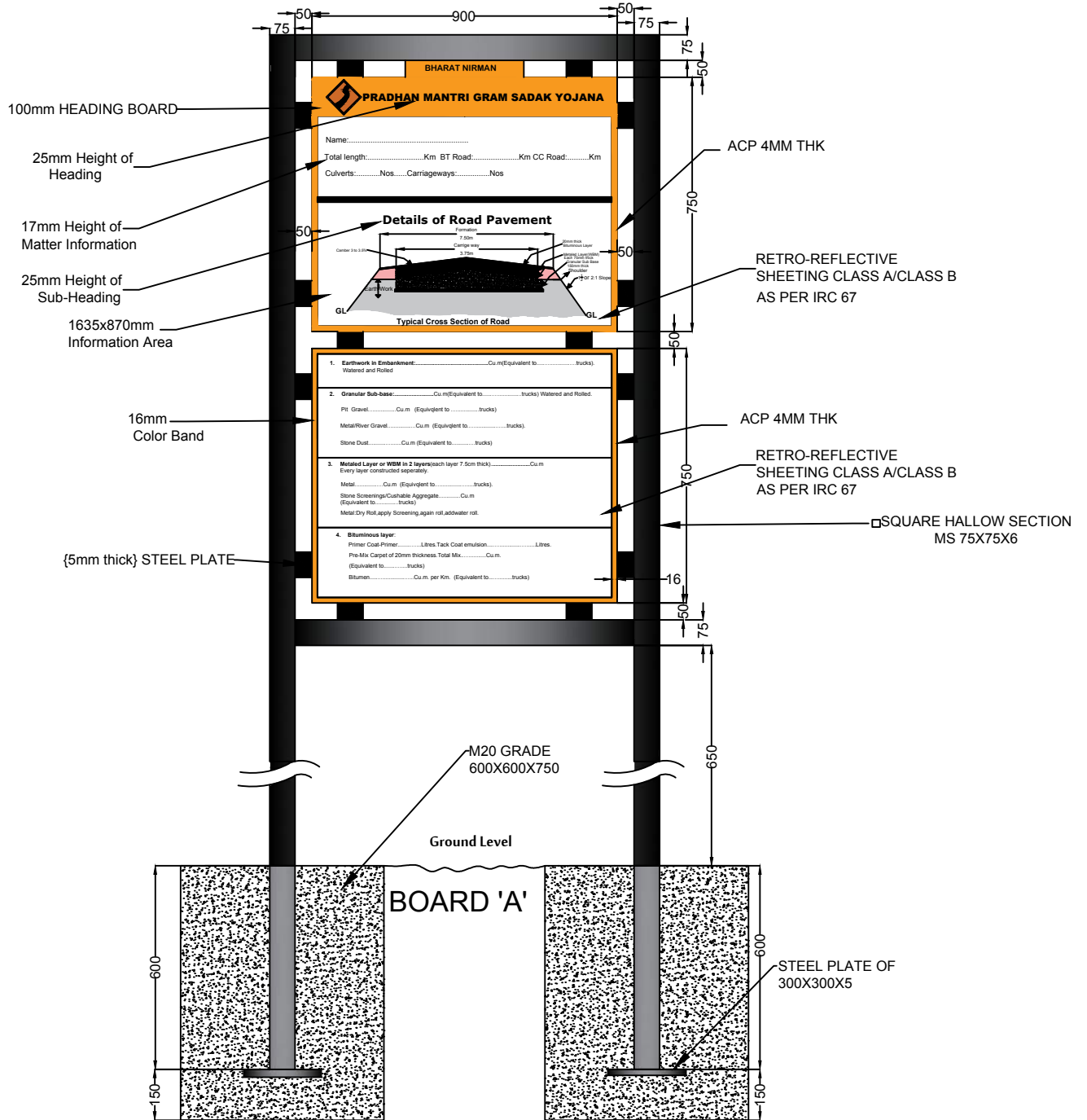
Fig.3 - CITIZEN INFORMATION BOARD "A"
