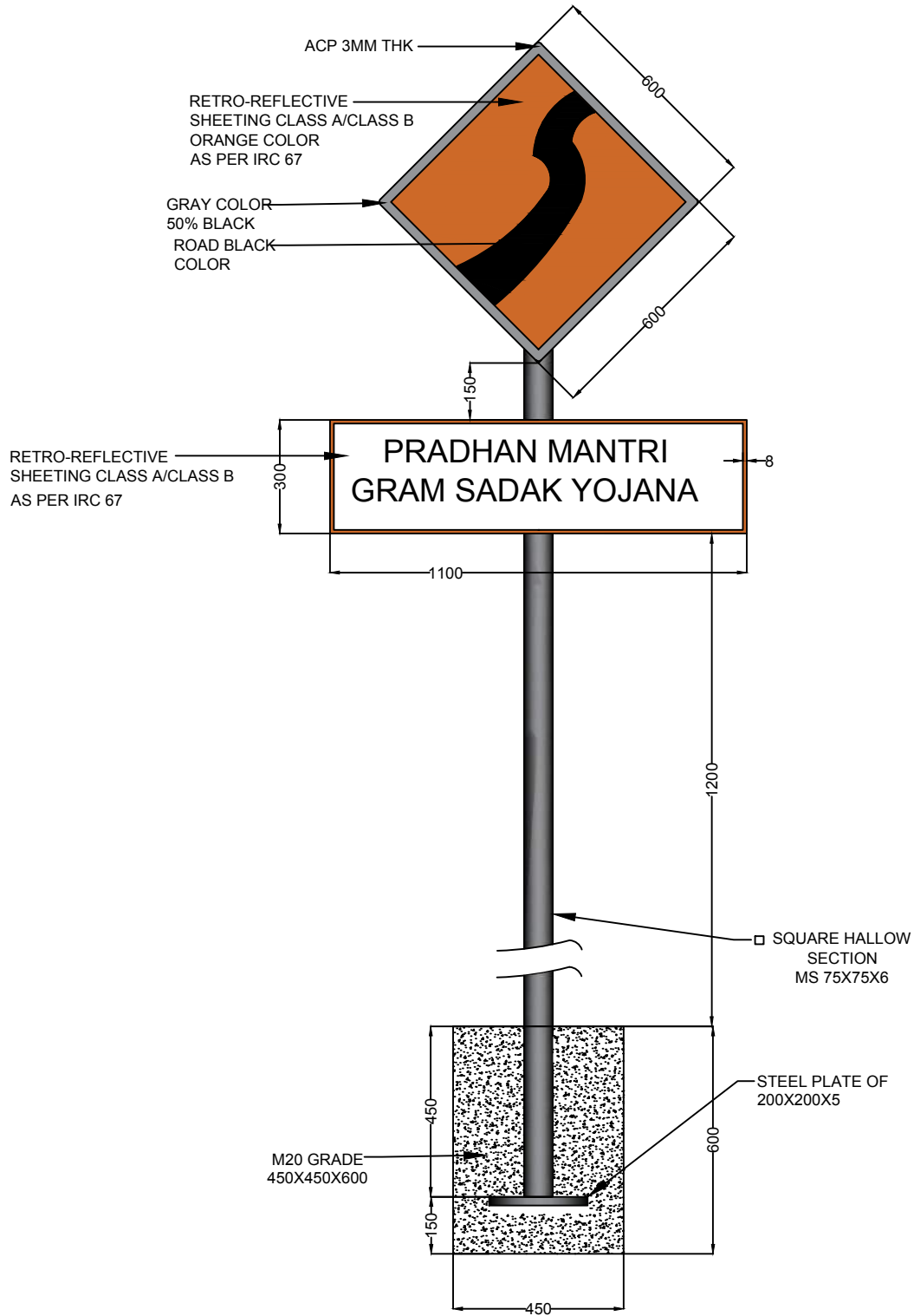
Fig.1(B) LOGO BOARD AT INTERMEDIATE DISTANCE
