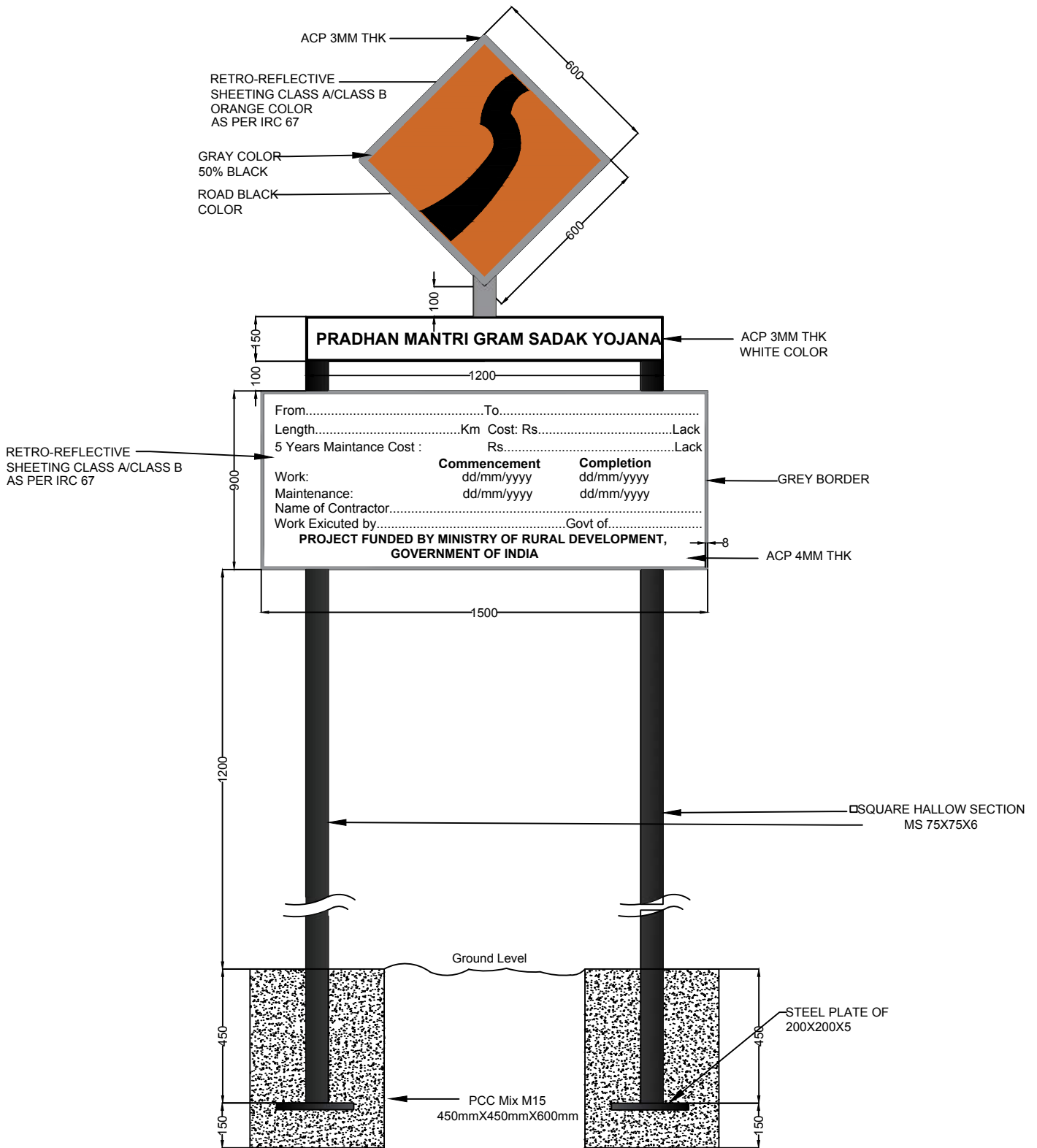
Fig.2-TYPICAL PMGSY LOGO AND INFORMATORY SIGN BOARD
